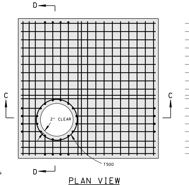
SECTION A-A X-SECT. VIEW IS PROVIDED ON STANDARD DRAWING D-CB-99 SHOWING REINFORCEMENT REQUIREMENTS AROUND PIPE OPENINGS
